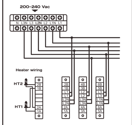
6 ZONES CONTROL CABINET WIRING DIAGRAM
