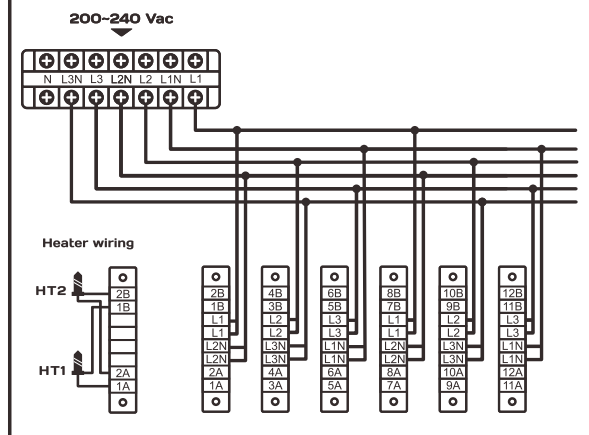
12 ZONES CONTROL CABINET WIRING DIAGRAM
